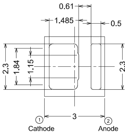
Bot. view
